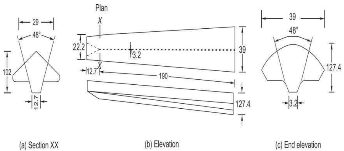
Two-way keys (dimensions in mm)
