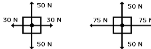
These two objects are at equilibrium since the forces are balanced. However, the forces are not equal.
