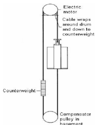
Traction Drum Arrangement
