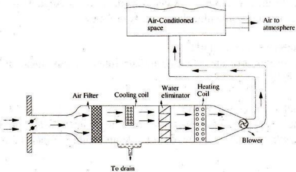
Fig. 2.29(a) Summer air-conditioning system
