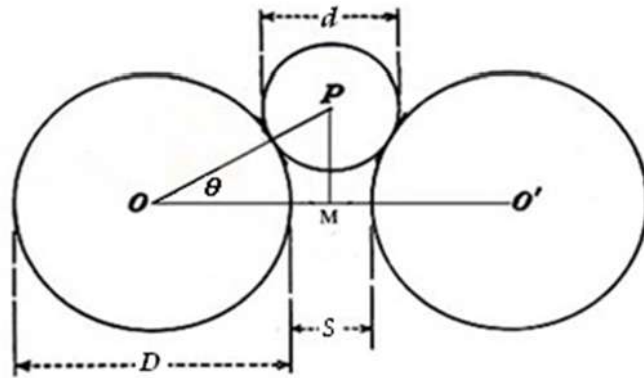
Fig.2.9. Inter-relationship between D, d, S and angle of nip ( \theta )
