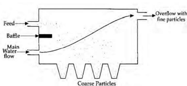
Fig.5.4. Richards Hindered Settler.
