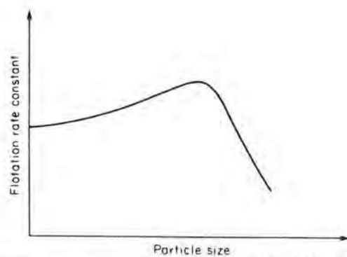
Rate of Flotation vs. Particle Size.
