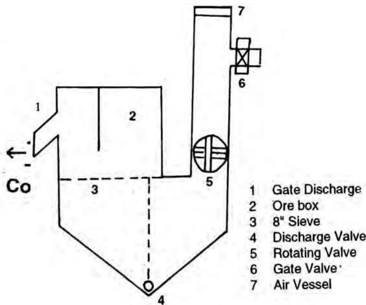
Pulsator Jig
