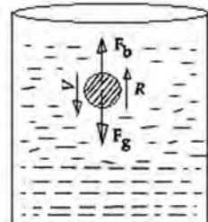
Forces acting on a Spherical particle under motion.
