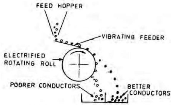
Electrostatic separator.
