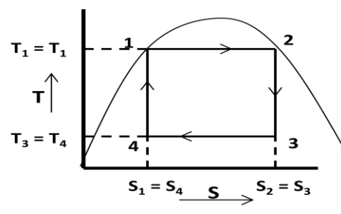
(T-s diagram)
