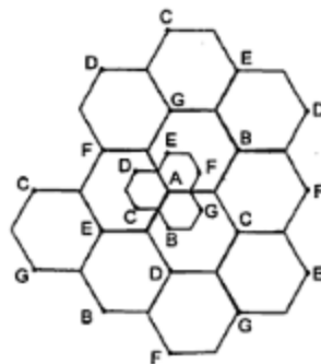
Fig. shows a cell splitting in which a congested cell, divided into smaller micro cells, and the base stations are put up at corners of the cells. The micro-cells are to be added in such a way
