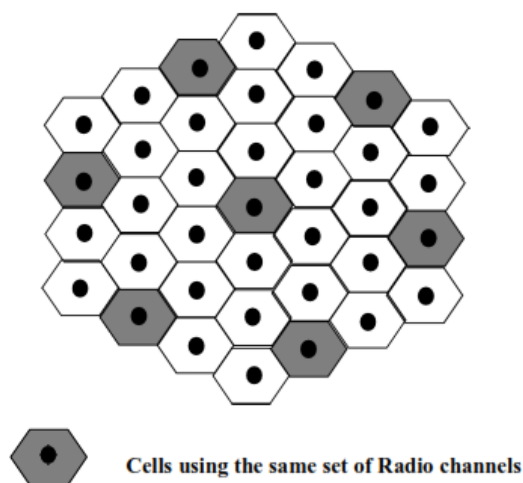
Figure 1. Cellular Network with Rrequency Reuse
