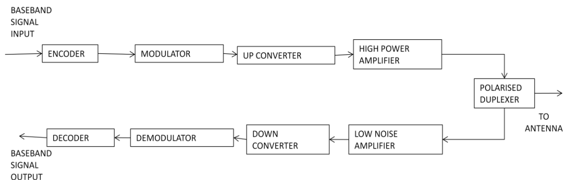
Block diagram of earth station
