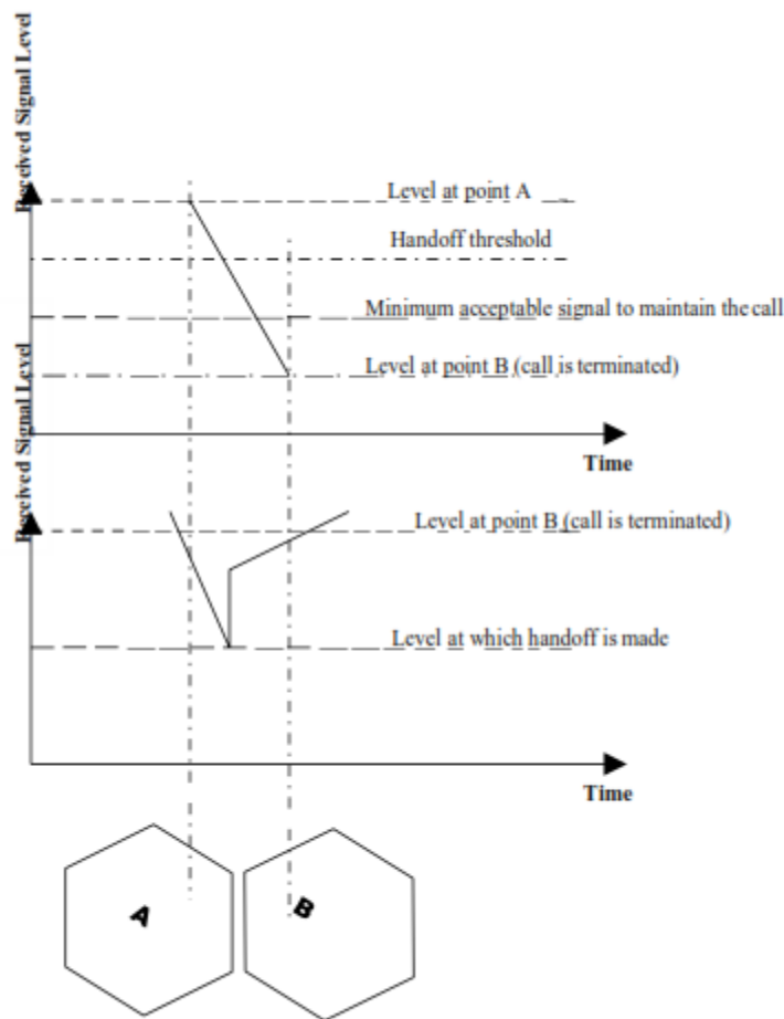
Fig. 1.11: Handoff Situation
