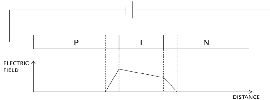
ELECTRIC FIELD DISTRIBUTION UNDER REVERSE BIAS
