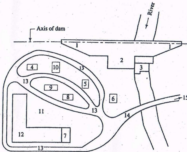
Job layout for dam site
