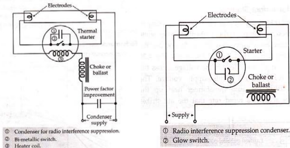
Fig.9 Fluorescent lamp
