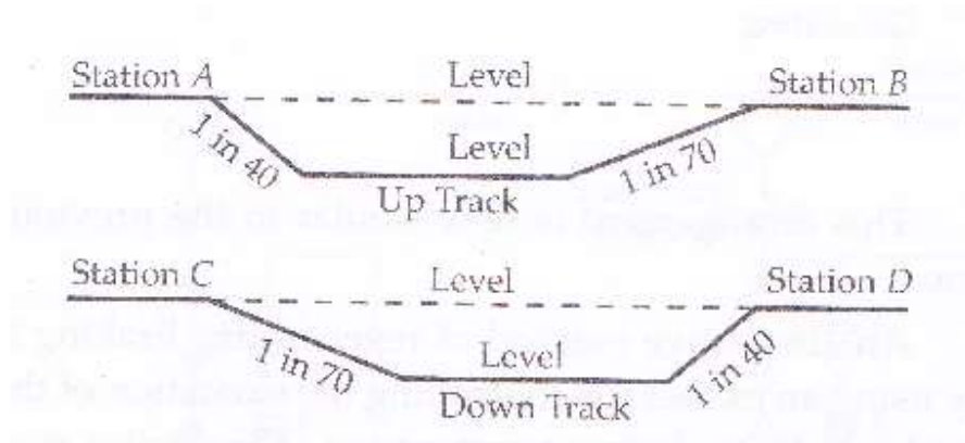
Fig.18 Track Grading
