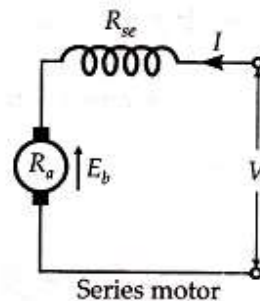
Fig. 1 DC series wound motor
