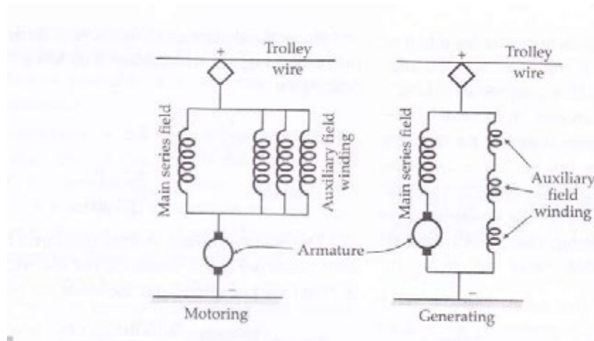
Fig. 20 Regenerative braking
