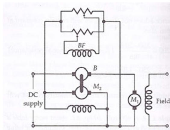
Fig.16 Booster control
