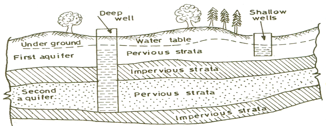
Fig. 3.5 (Shallow & deep well)
