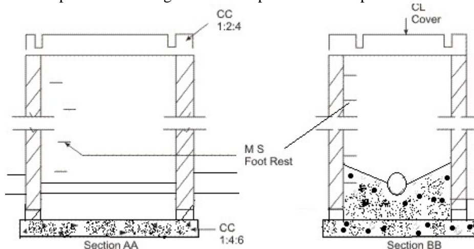
Shallow Manhole
