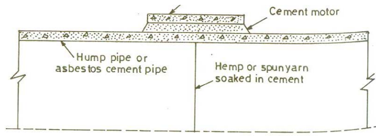
Fig. 4.9 (Collar Joint)
