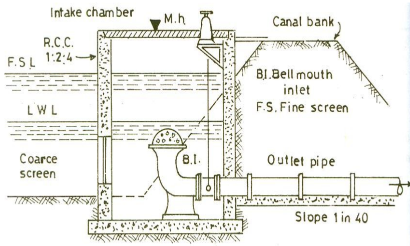
Fig. 4.4 (Canal Intake)
