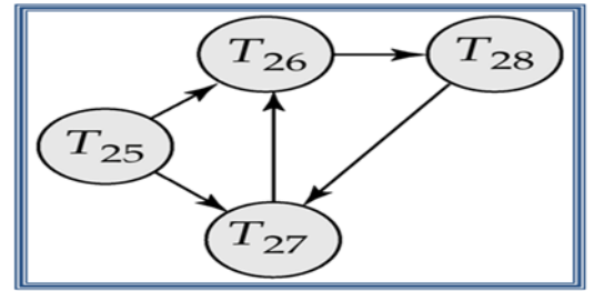
Wait-for graph with a cycle
