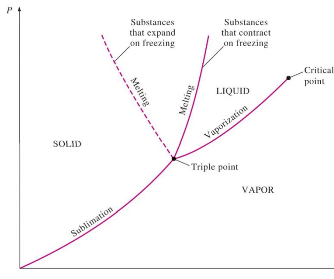
P-T diagram and the triple point.
